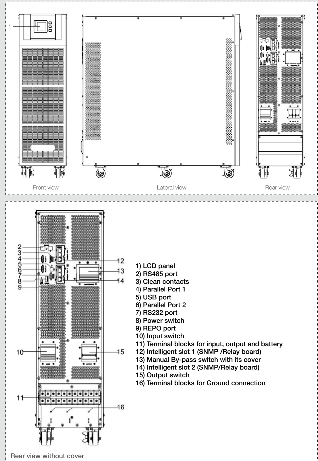
Figure 1: cabinet UPS
